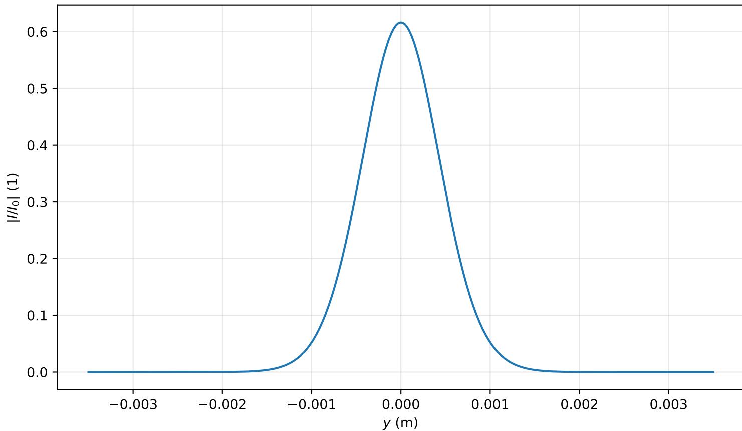
Intensity profile I(x=0, y, z=1.911)/I_0 , P_{in}=0.2P_{cr} , artificial time
